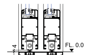
Flush Track
