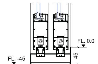
Common Track
